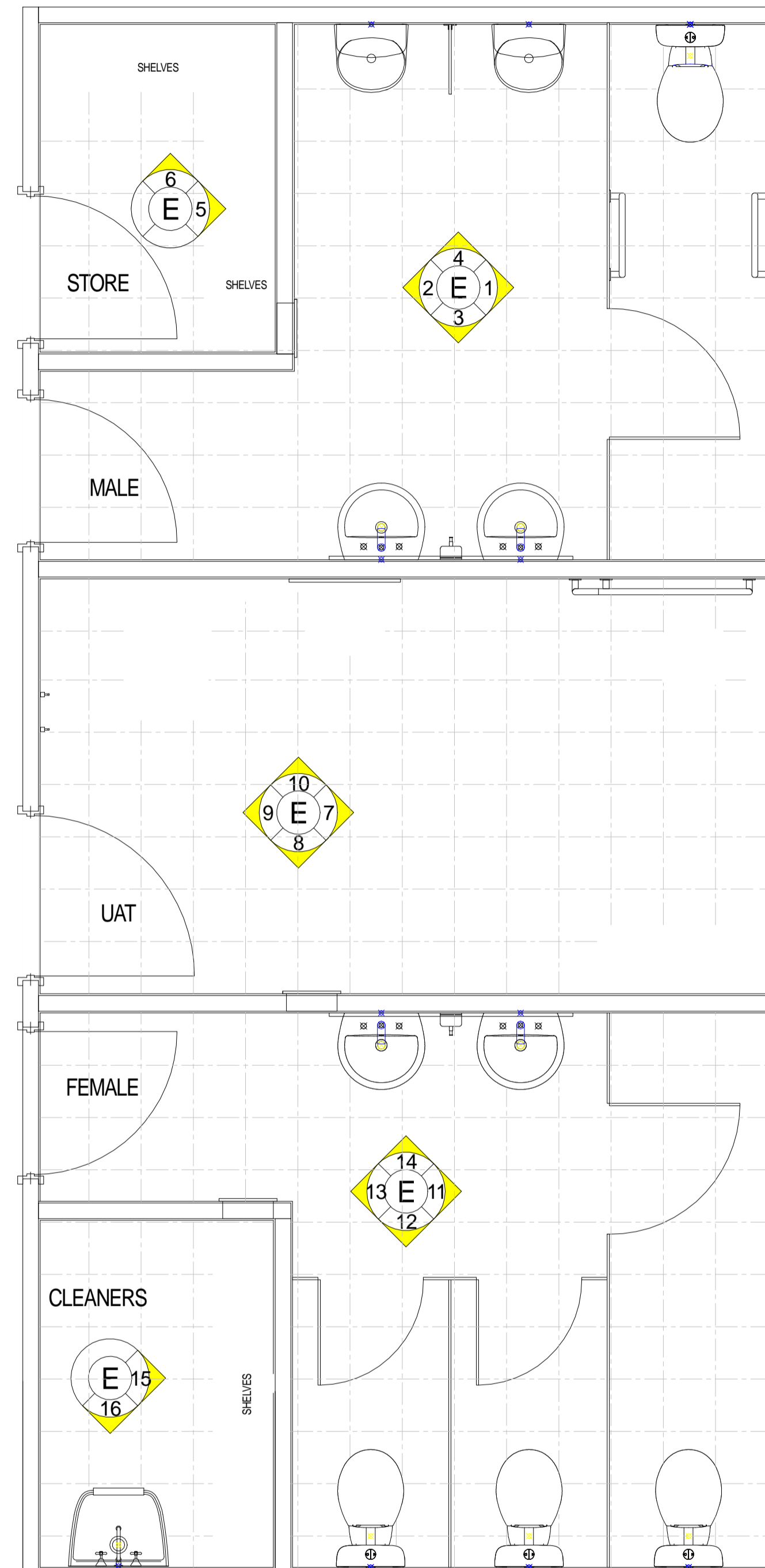
P N AMENITIES FLOOR PLAN SCALE 1:25
