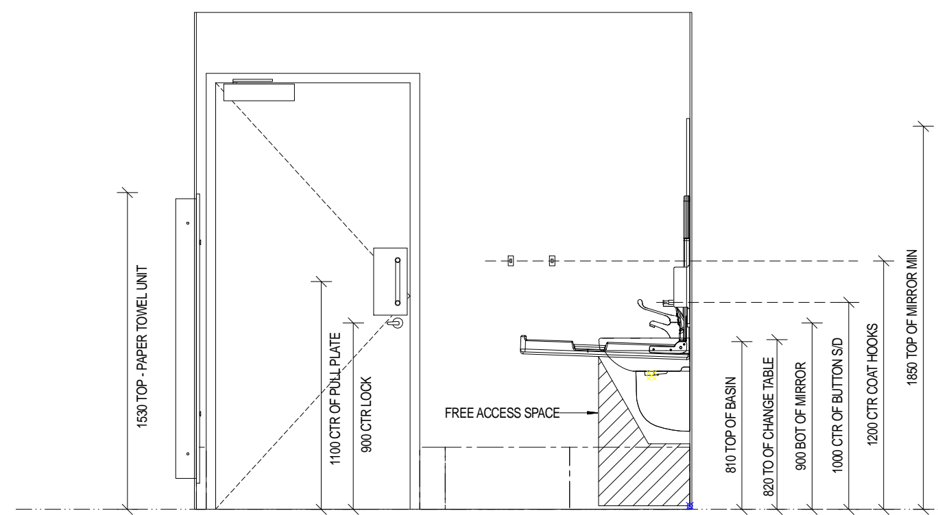
9 AMENITIES INT ELEV SCALE 1:25 A151
