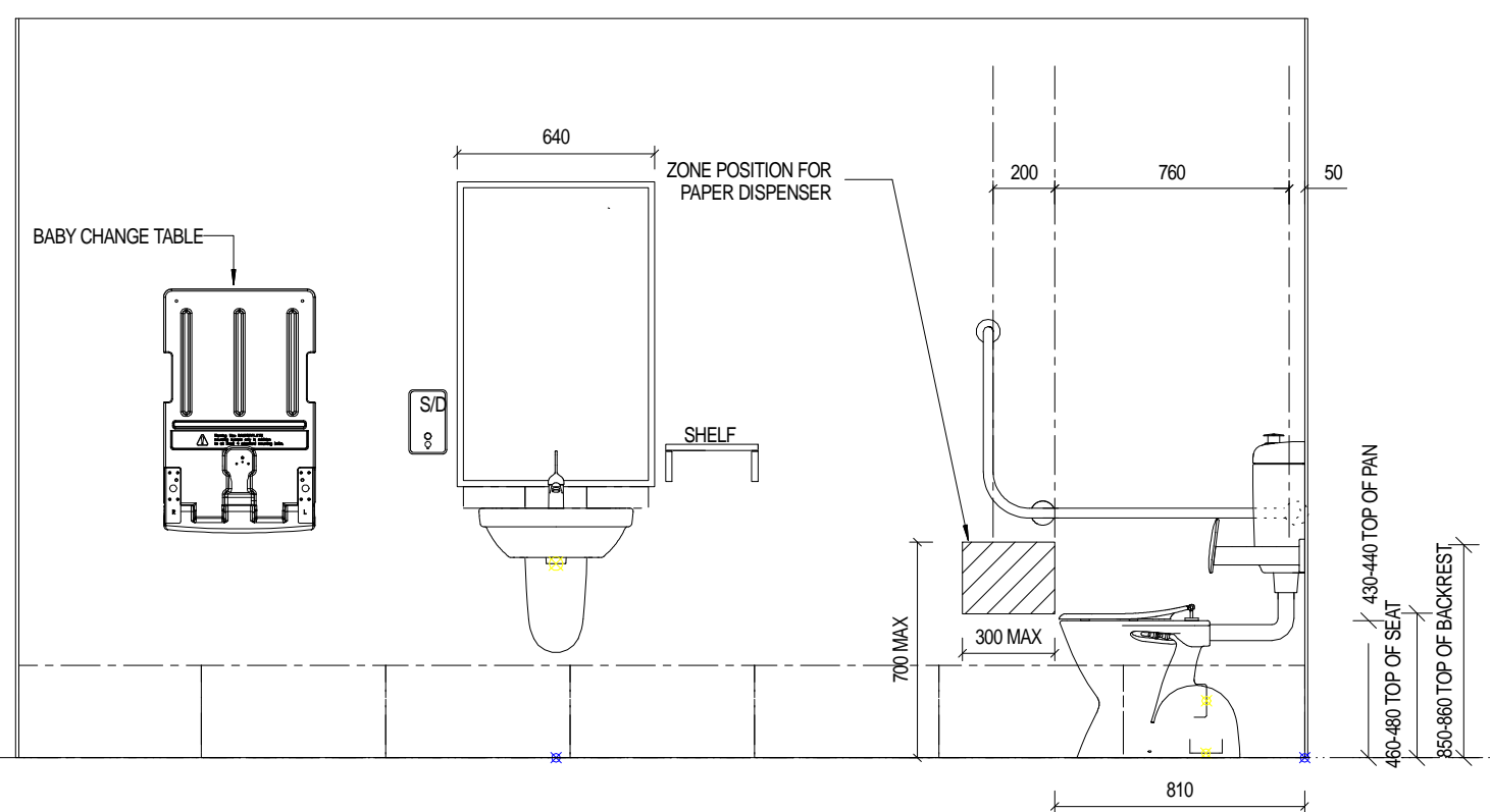
10 AMENITIES INT ELEV SCALE 1:25 A151
