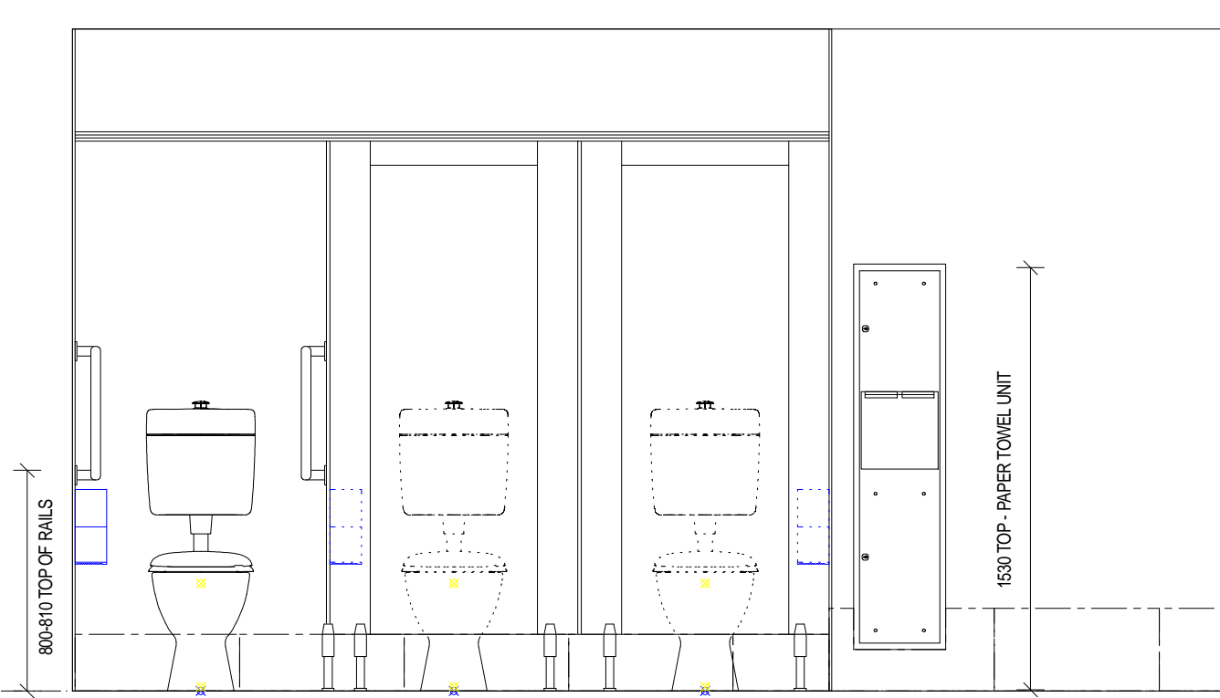
12 AMENITIES INT ELEV SCALE 1:25 A151
