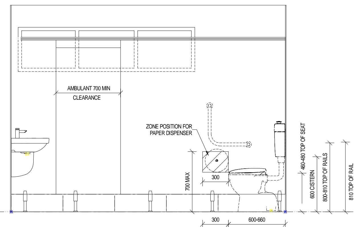
11 AMENITIES INT ELEV SCALE 1:25 A151
