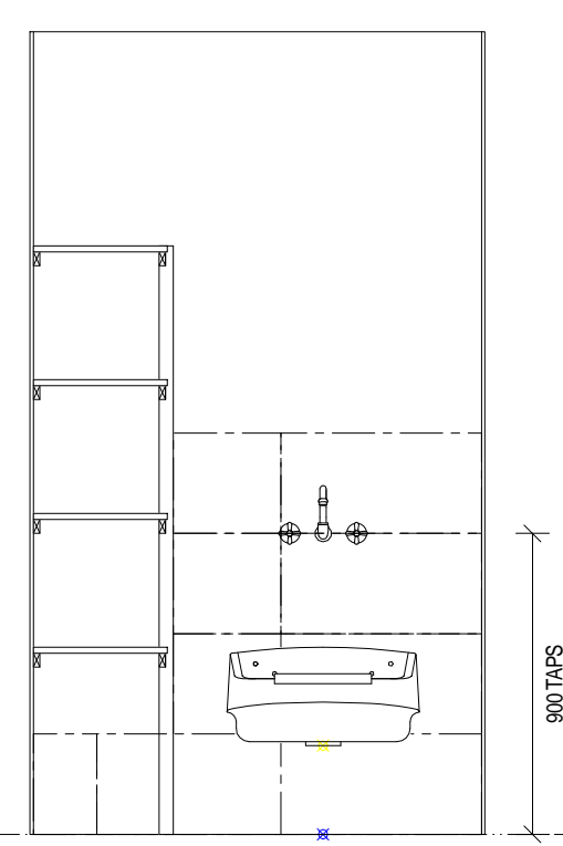
16 AMENITIES INT ELEV SCALE 1:25 A151
