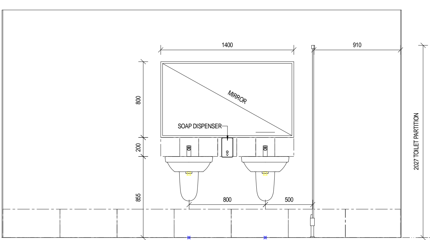
14 AMENITIES INT ELEV SCALE 1:25 A151
