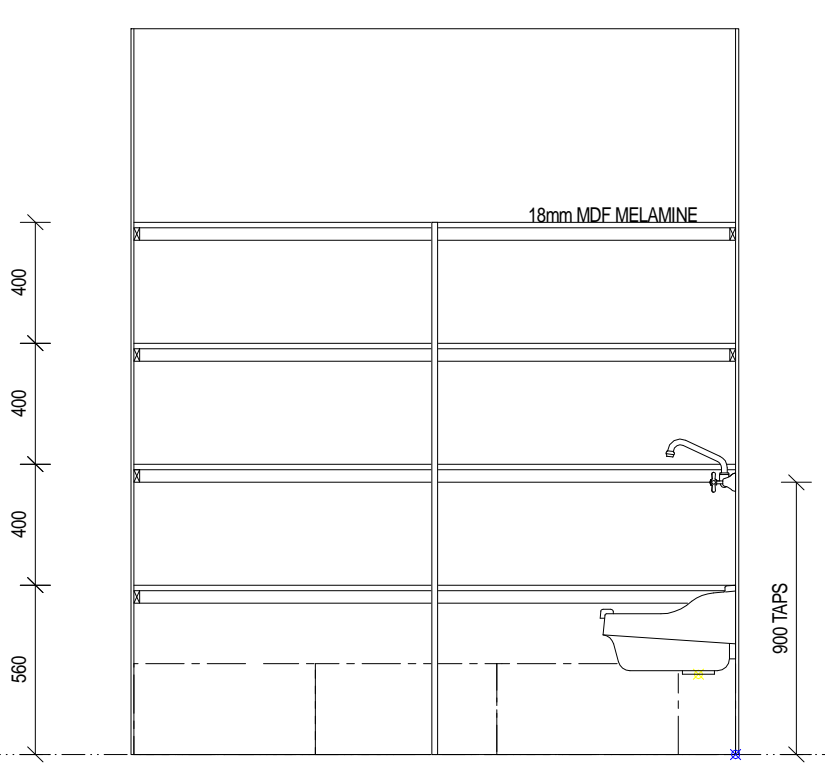
15 AMENITIES INT ELEV SCALE 1:25 A151
