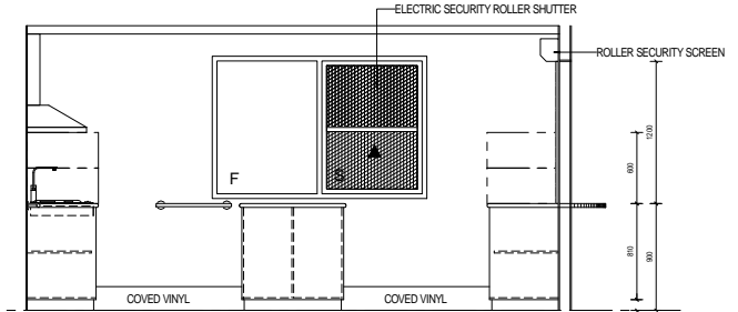
19 KITCHEN INT ELEV SCALE 1:25
