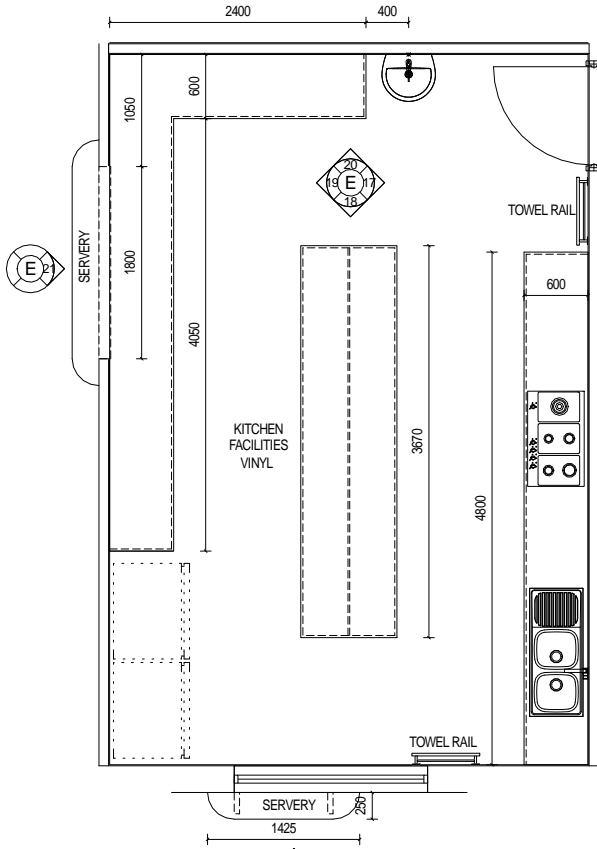
20 KITCHEN FLOOR PLAN SCALE 1:25
