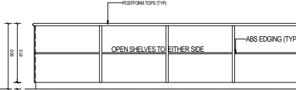
18 KITCHEN ISLAND ELEV SCALE 1:25
