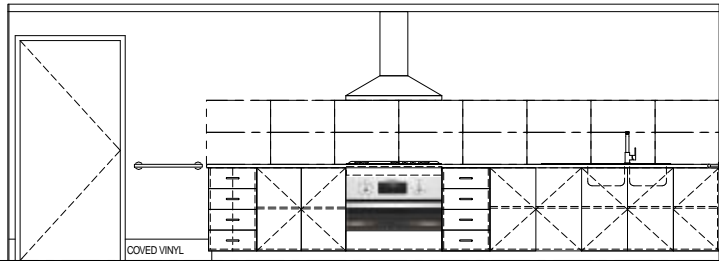
17 KITCHEN INT ELEV SCALE 1:25
