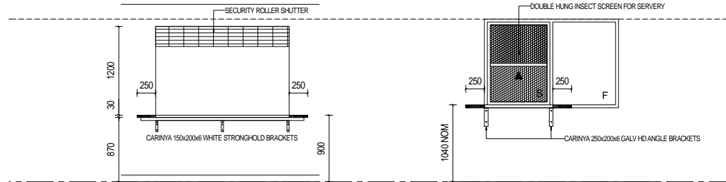
21 KITCHEN INT ELEV SCALE 1:25
