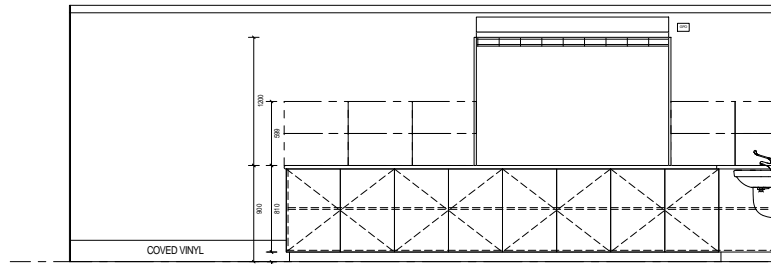
17 KITCHEN INT ELEV SCALE 1:25
