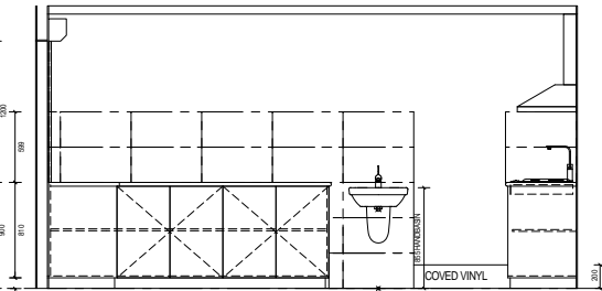
18 KITCHEN INT ELEV SCALE 1:25
