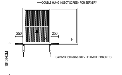
22 KITCHEN INT ELEV SCALE 1:25
