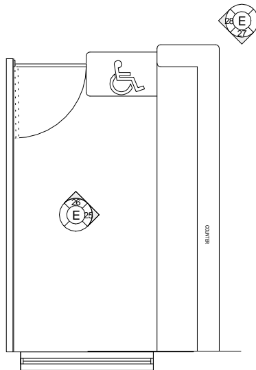
COUNTER FLOOR PLAN SCALE 1:25
