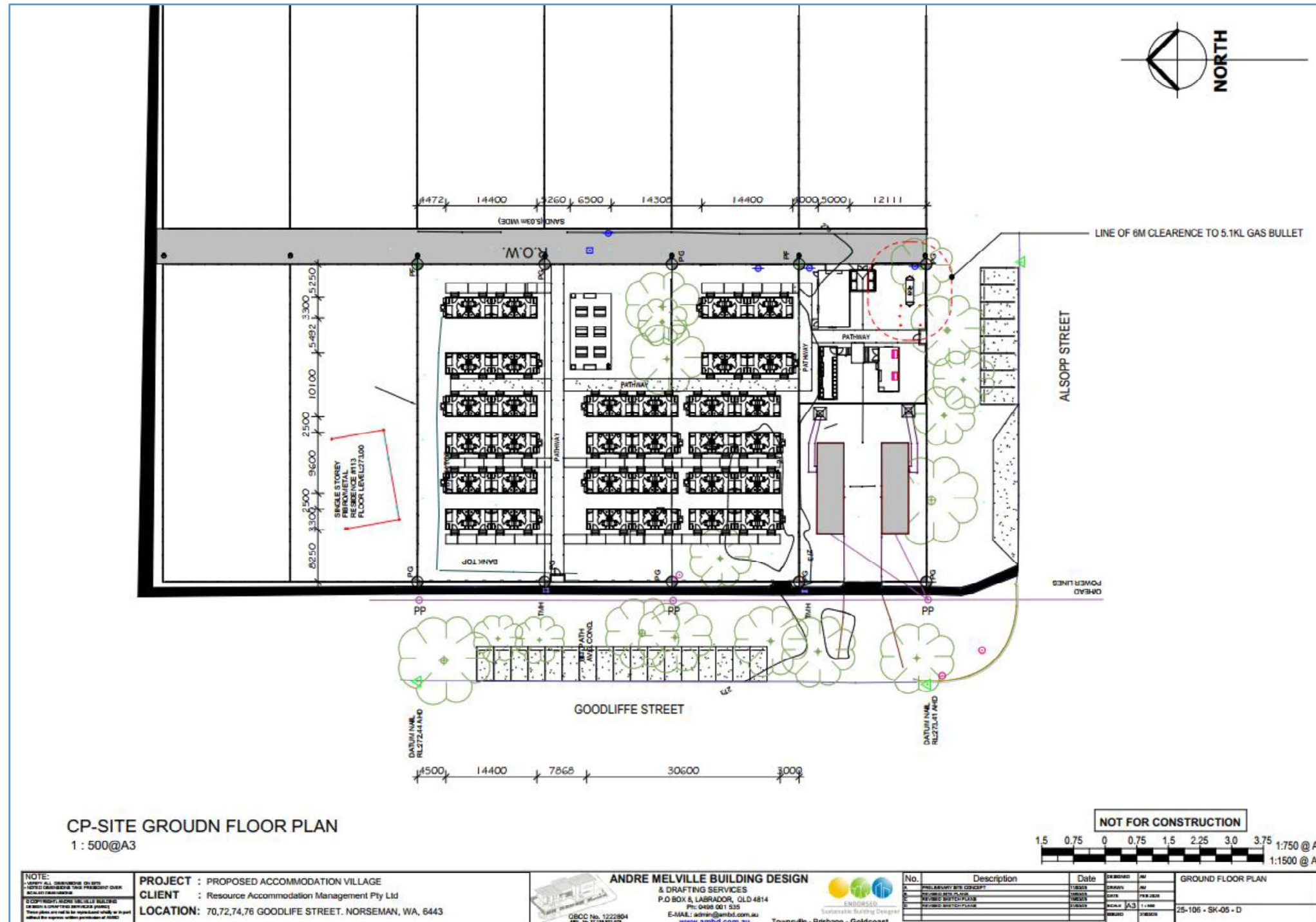
Figure 3: Site Layout
